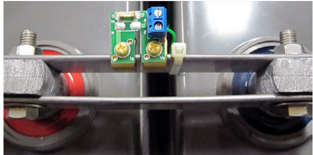
C-Type Clamps Installed to Busbars
