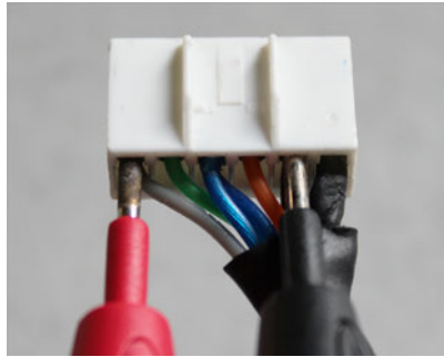
Test Connection between Clamp 1 & Clamp 5 of 12V Cells
