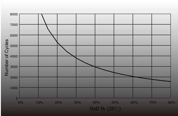
Cycle Life in Relation to DOD
