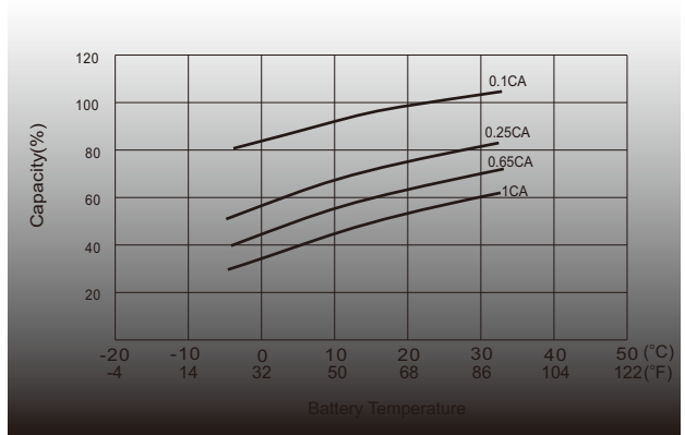
Temperature effects in relation to battery capacity
