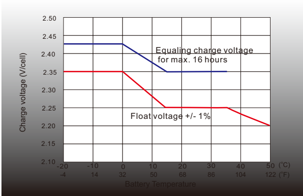
Charge voltage vs ambient temperature curve
