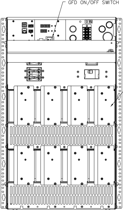
CHARGER SHOWN WITH DOOR OPEN, UIM ACCESS
