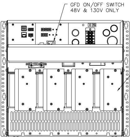
CHARGER SHOWN WITH DOOR OPEN, UIM ACCESS
