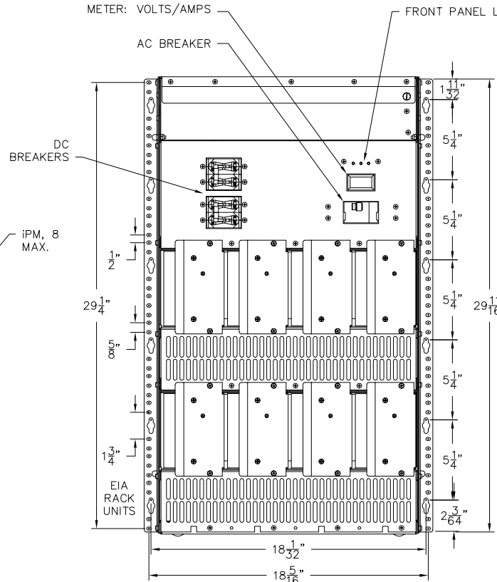
CHARGER SHOWN WITH DOOR OPEN, UIM ACCESS
