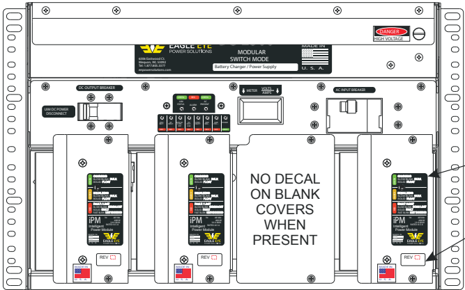
CHARGER FRONT VIEW
